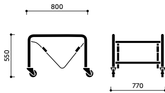
W (chairs trolley)
