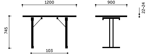
Standard Folding Table 4680-15
