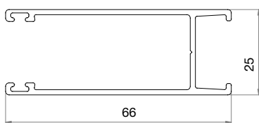
Nischmontering MEDIUM, LARGE
